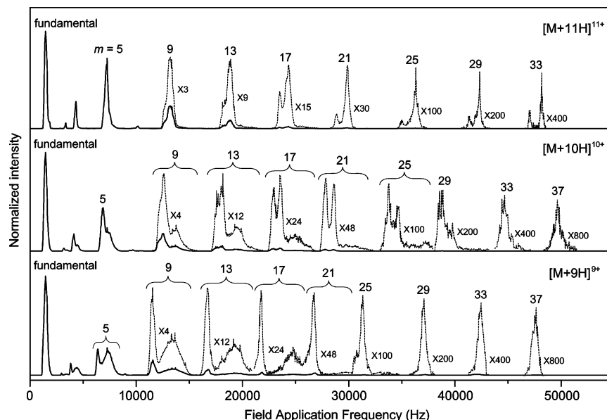
Figure 2. Experimental OMS distributions for the [M+9H]^{9+} to [M+11H]^{11+} charge states of electro sprayed ubiquitin ions. The data are plotted as a function of field application frequency over a range of 0 to 55000 Hz. Low intensity features of each charge state are magnified (dashed lines). m indicates the harmonic frequency number permitting ion transmission (see text for details).
