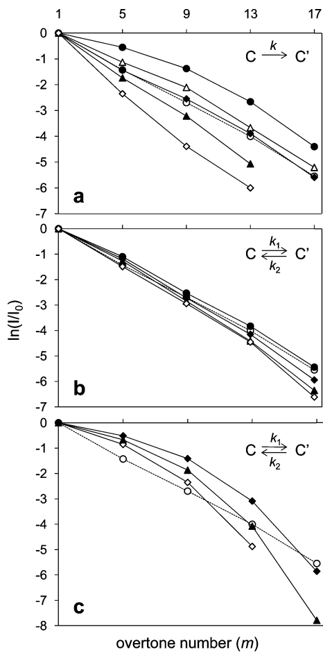
Figure 7. Plot of calculated and experimental relative intensity ratios as a function of m for a partially folded conformation (labeled C in Figure 5) of the [M+9H]^{9+} charge state of ubiquitin ions. The dashed trace represents relative intensities obtained from the experimental results. Relative intensities obtained from ion trajectory simulations were calculated utilizing \pm 4\% variation in mobility (see text for details). The three kinetics models used to simulate the intensities of conformer C during ion transmission are as follows: (a) an irreversible reaction ( \bullet k = 10 ; \triangle k = 100 ; \blacklozenge k = 150 ; \circ exp.; \blacktriangle k = 200 ; \diamond k = 300 ); (b) a reversible reaction at relatively low rates ( k_1 = 200 for all; \bullet k_2 = 200 ; \circ exp.; \blacklozenge k_2 = 150 ; \blacktriangle k_2 = 100 ; \diamond k_2 = 50 ); (c) a reversible reaction at relatively high rate constant ( k_1 = k_2 ; \blacklozenge k = 6932 ; \circ exp.; \blacktriangle k = 2310 ; \diamond k = 1155 ).
