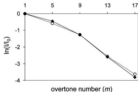
Figure 6. Plot of calculated ( \blacklozenge ) and experimental ( \circ ) relative intensity ratios as a function of m for the elongated conformation (labeled A in Figure 5) of the [M+9H]^{9+} charge state of ubiquitin ions. Relative intensities obtained from ion trajectory simulations were calculated accounting for a contribution from ion diffusion but excluding structural transitions.
