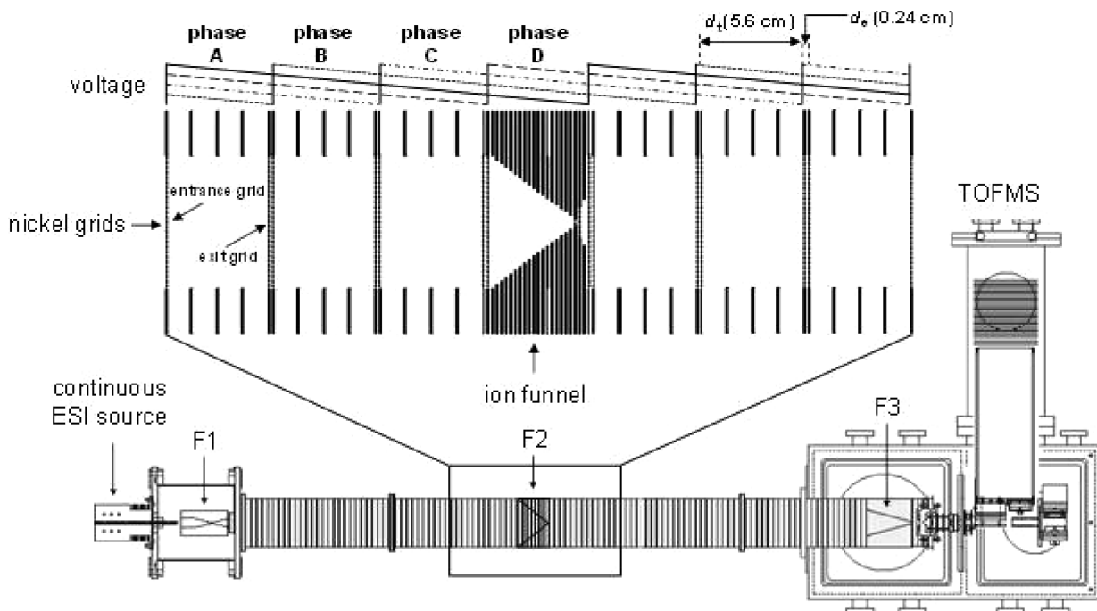
Figure 1. Schematic diagram of the OMS-TOF instrument used to measure the collision cross section distributions. The drift tube assembly consists of three ion funnels (F1–F3) and multiple segmented drift regions (22 sections). The segmented regions are divided by lenses containing nickel mesh grids. Each section is operated using an electric field of 9 \text{ V} \cdot \text{cm}^{-1} (ion transmission region, 5.6 cm). Periodic repulsive fields of 963 \text{ V} \cdot \text{cm}^{-1} are created between specific sets of grids ( d_e regions, 0.24 cm). The four-phase system applied in these studies utilizes four distinct drift field settings (phases A, B, C, and D). These fields are modulated at different frequencies to allow the ions with appropriate mobilities to move through the drift tube.
