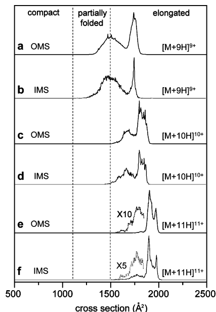
Figure 3. Cross section distributions for the [M+9H]^{9+} to [M+11H]^{11+} charge states of ubiquitin ions obtained from OMS (a, c, and e) and IMS (b, d, and f) measurements. For OMS distributions, the 9\cdot f_i , 13\cdot f_i , and 17\cdot f_i overtone spectra have been chosen for the [M+9H]^{9+} , [M+10H]^{10+} , and [M+11H]^{11+} ions, respectively. Regions divided by dashed lines correspond to compact, partially folded, and elongated conformations, as defined previously. 56 IMS distributions are obtained by taking slices from a two-dimensional t_D(m/z) data set. The OMS distributions are plotted by determining the cross sections from overtone frequencies, eq 1.
