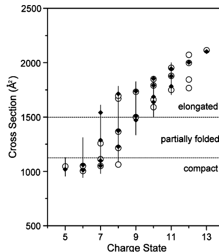
Figure 4. Cross sections for the [M+5H]^{5+} to [M+13H]^{13+} charge state ions of ubiquitin. The open circles correspond to data recorded using IMS. 59 The solid diamonds indicate data obtained by OMS. The vertical lines show a range of cross sections that are associated with unresolved conformations. Dashed lines indicate divisions for compact, partially folded, and elongated conformational states. Different overtone spectra for individual charge states have been analyzed to calculate the cross sections (the 5\cdot f_i overtone spectra for the [M+5H]^{5+} to [M+8H]^{8+} ions, the 9\cdot f_i overtone spectrum for the [M+9H]^{9+} ions, the 13\cdot f_i overtone spectrum for the [M+10H]^{10+} ions, and the 17\cdot f_i overtone spectra for the [M+11H]^{11+} to [M+13H]^{13+} ions).
