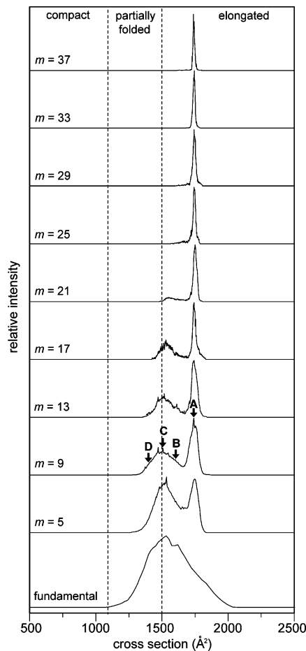
Figure 5. Cross section distributions for the [M + 9H]^{9+} charge state of electro sprayed ubiquitin ions obtained from OMS measurements. The OMS spectrum has been recorded from the f_i to the 37 \cdot f_i overtone. m indicates the harmonic frequency number allowing the ion transmission. Dashed lines indicate divisions for compact, partially folded, and elongated conformational states. Four conformations (labeled A, B, C, and D, \Omega = 1417, 1508, 1612, and 1741 \text{ \AA}^2 , respectively) have been chosen to simulate structural transitions (see Figures 6 and 7 and the text for details).
